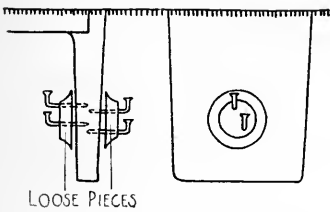
FIG. 576. LOOSE PIECE PATTERNS.
